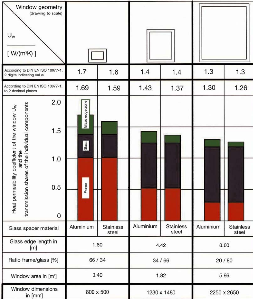
Fig. 2: Window U values depending on window size. Thermal input data: U_f = 1.5 W/(m^2K) , U_g = 1.1 W/(m^2K) , \psi_{Aluminium} = 0.075 W/(mK) , \psi_{Stainless steel} = 0.050 W/(mK) , geometry: Frame view width = 125 mm.
